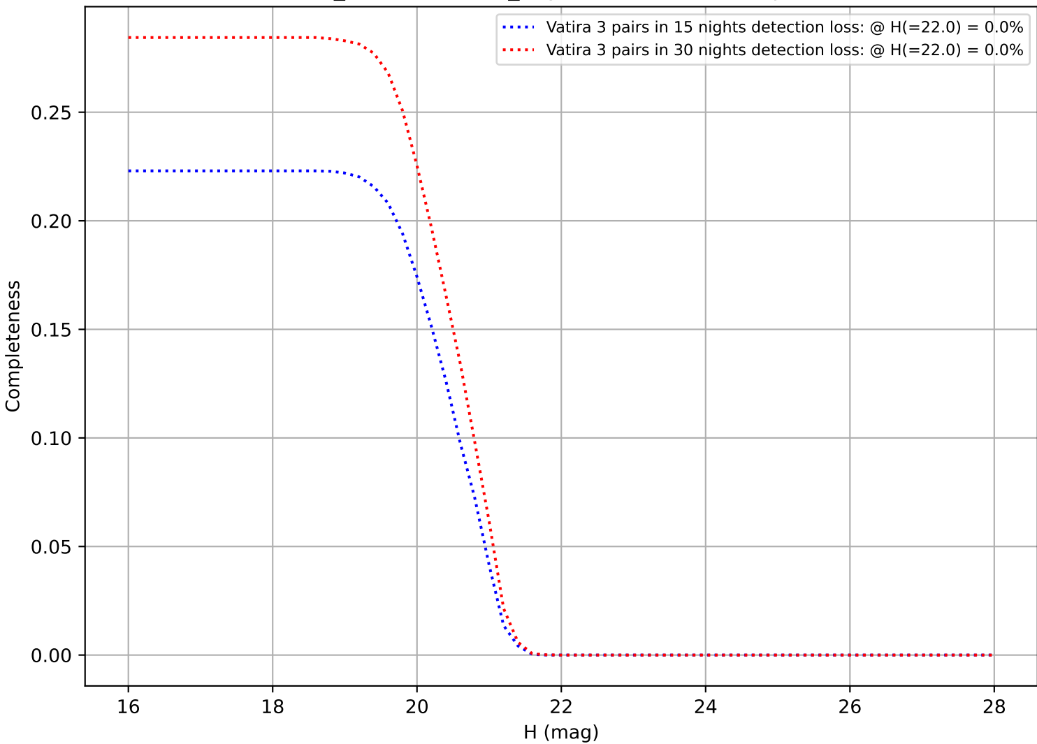
weather_cloudso31v3.4_10yrs: DifferentialCompleteness
