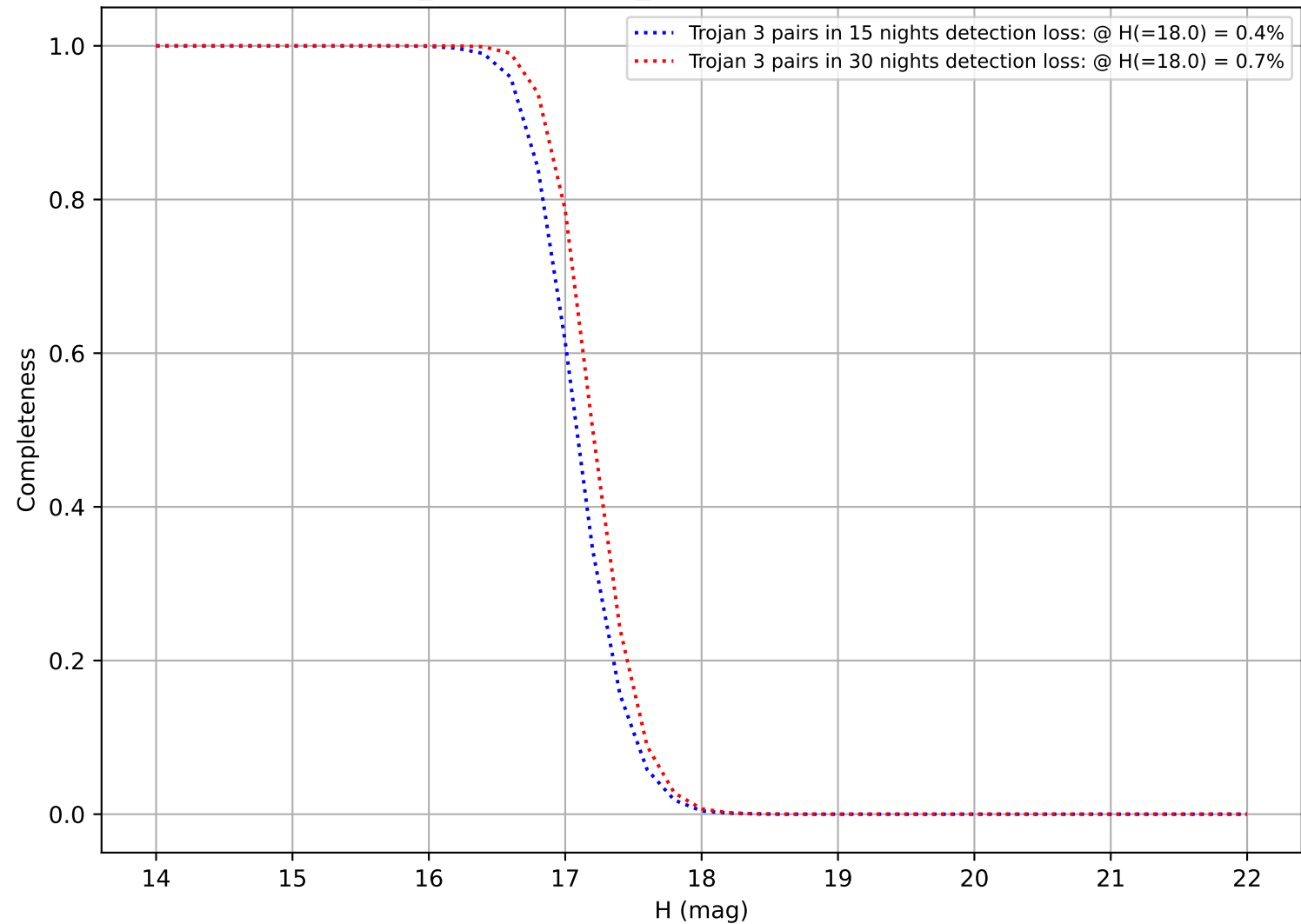
weather_cloudso31v3.4_10yrs: DifferentialCompleteness
