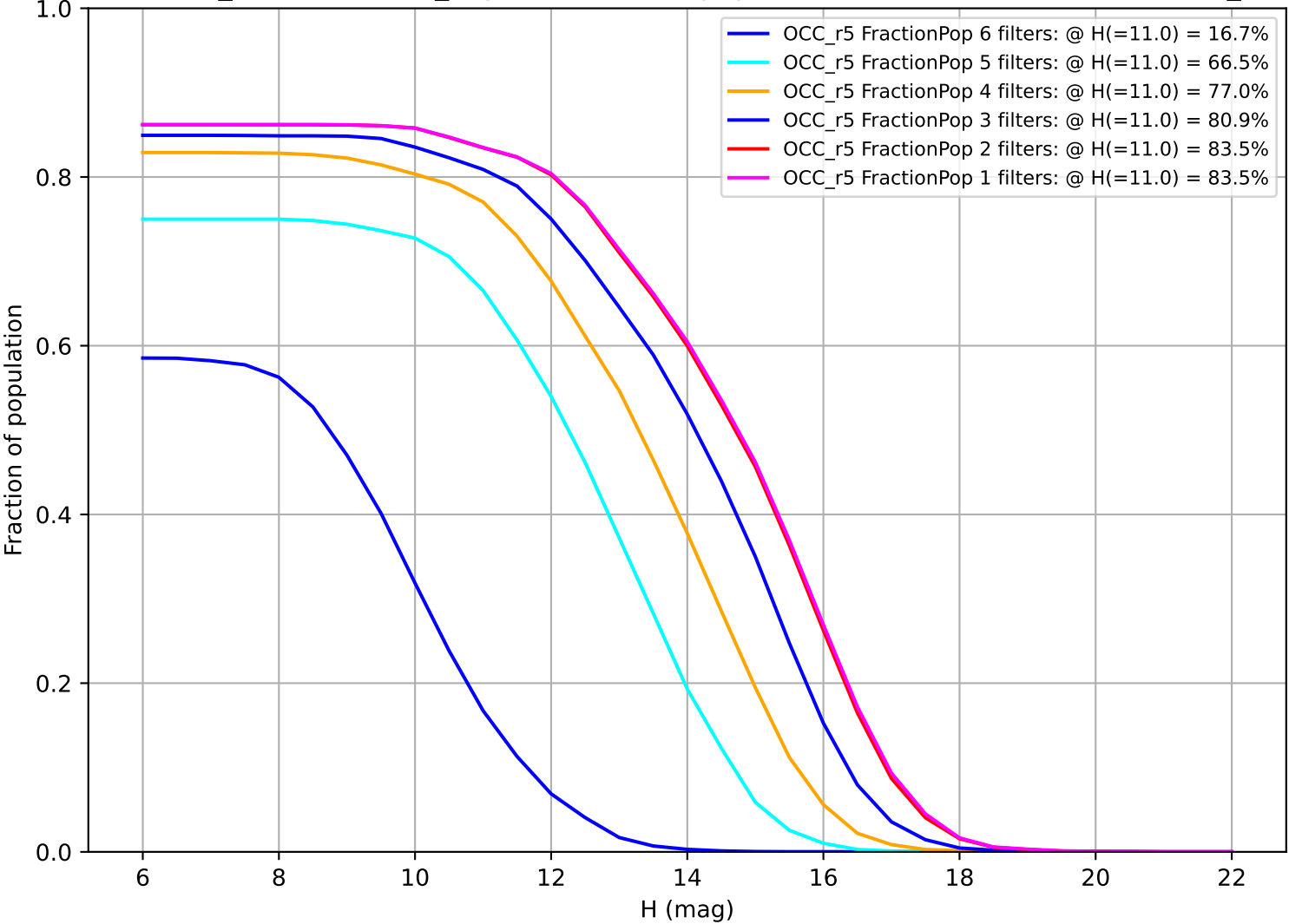
weather_cloudso31v3.4_10yrs: Fraction of population with colors in X filters OCC_r5
