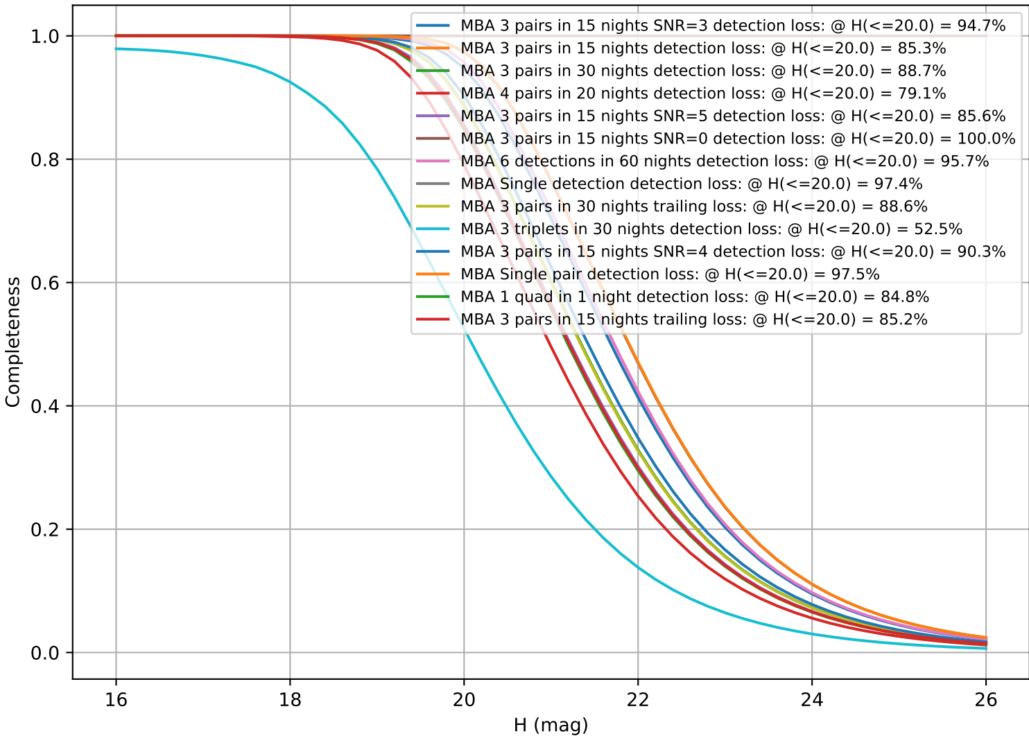
weather_cloudso31v3.4_10yrs: CumulativeCompleteness
