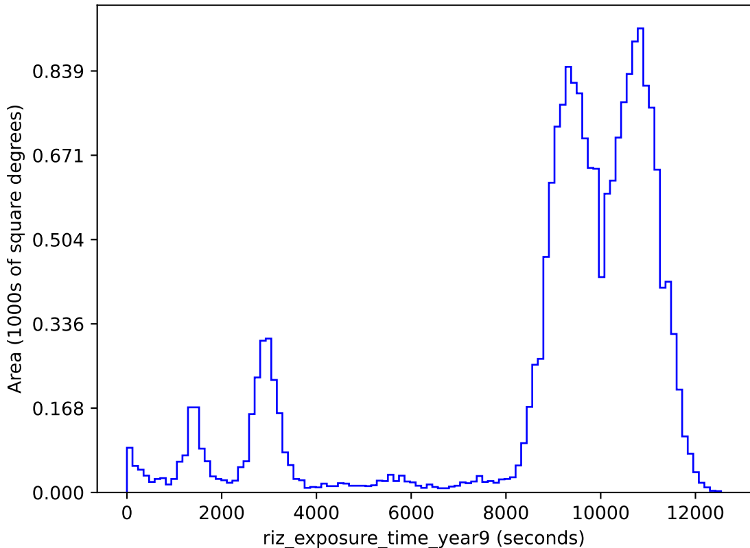
weather_cloudso31v3.4_10yrs gri band non-DD: riz_exposure_time_year9
