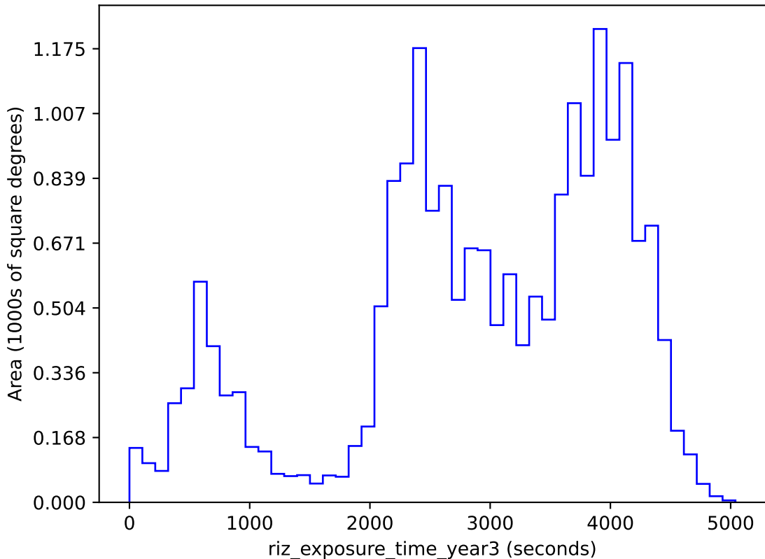
weather_cloudso31v3.4_10yrs gri band non-DD: riz_exposure_time_year3
