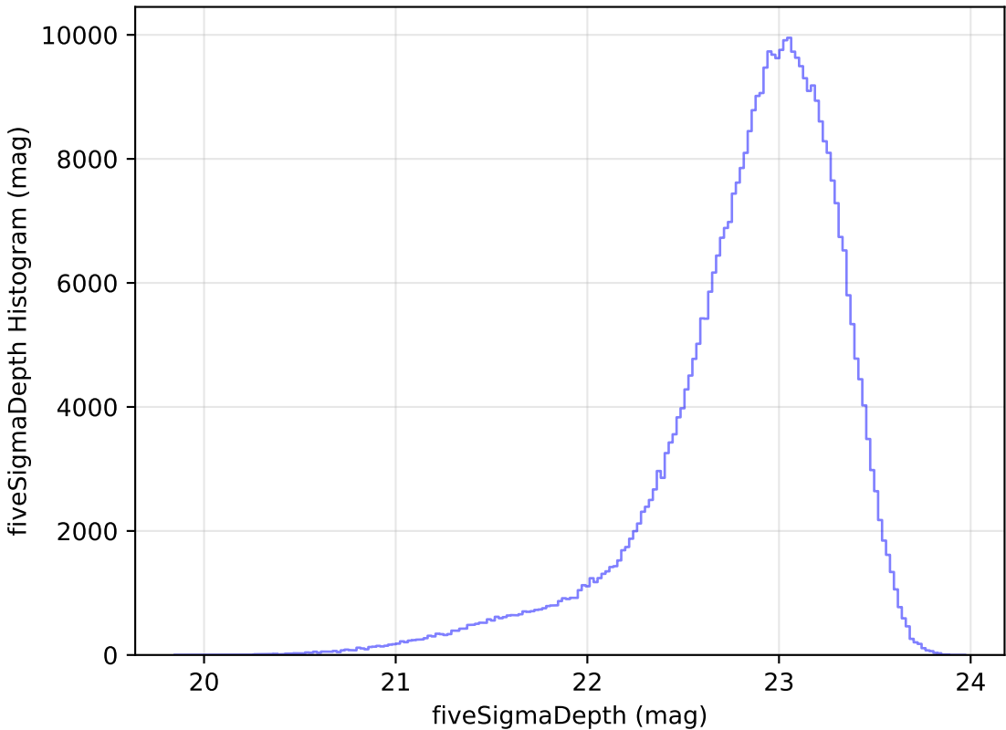
weather_cloudso31v3.4_10yrs z: fiveSigmaDepth Histogram
