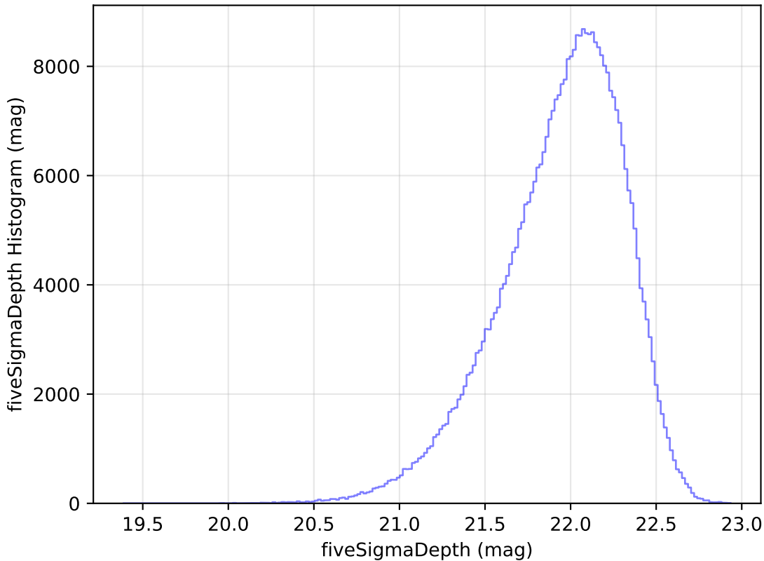
weather_cloudso31v3.4_10yrs y: fiveSigmaDepth Histogram
