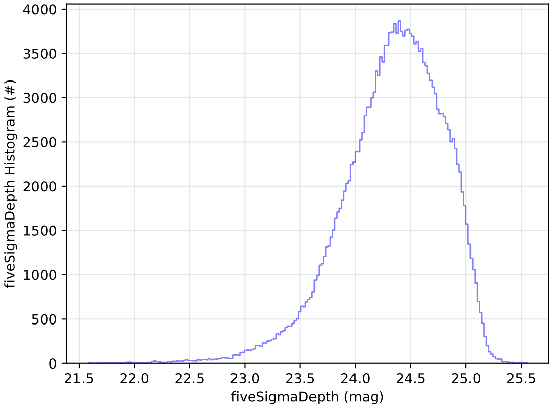
weather_cloudso31v3.4_10yrs g: fiveSigmaDepth Histogram
