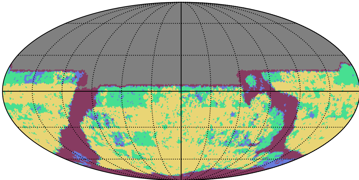
weather_cloudso31v3.4_10yrs u band: YearCoverage night
