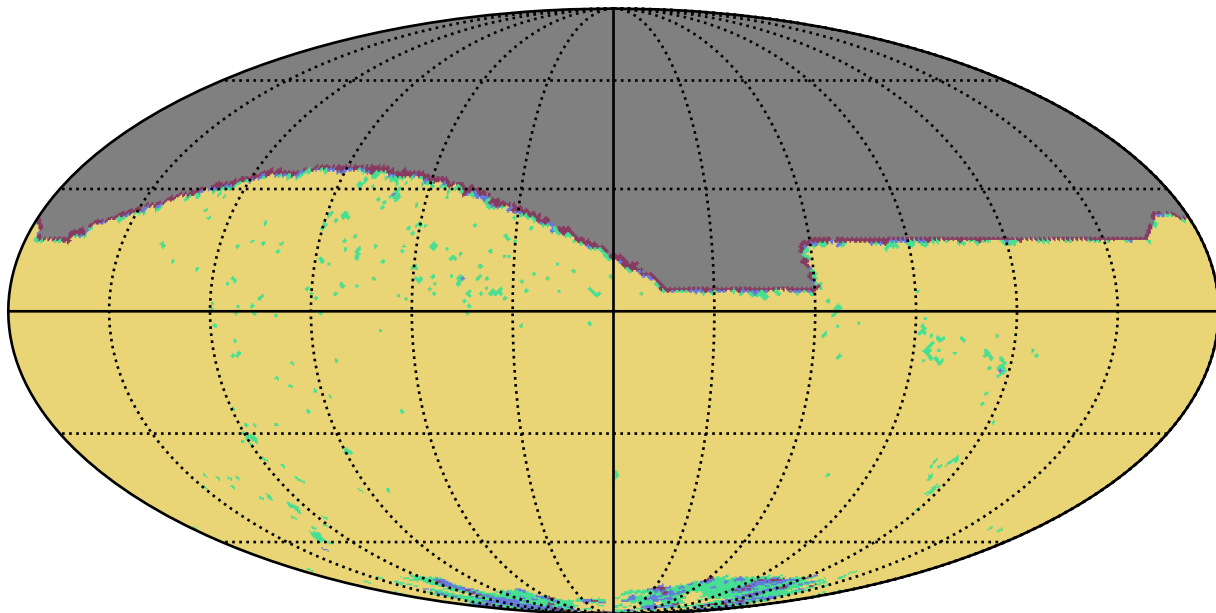
weather_cloudso31v3.4_10yrs i band: YearCoverage night
