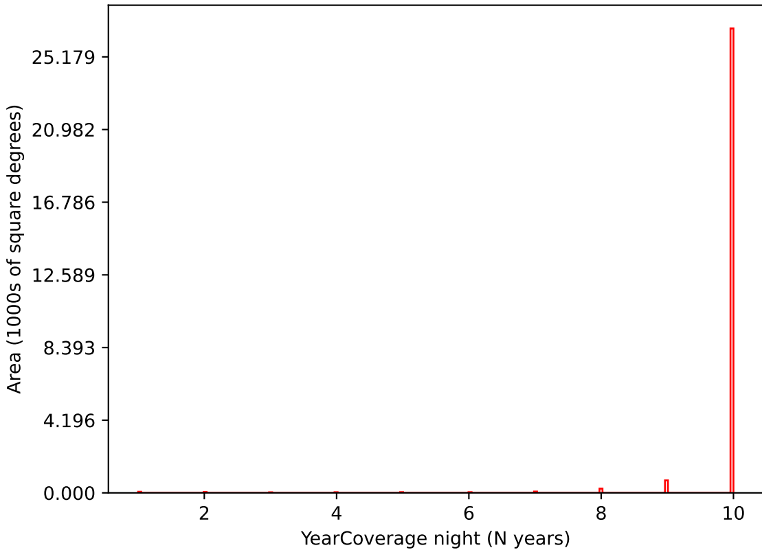
weather_cloudso31v3.4_10yrs i band: YearCoverage night
