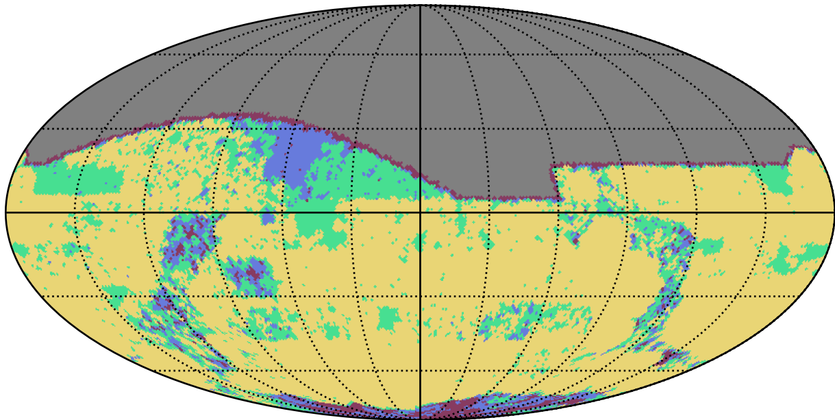
weather_cloudso31v3.4_10yrs g band: YearCoverage night
