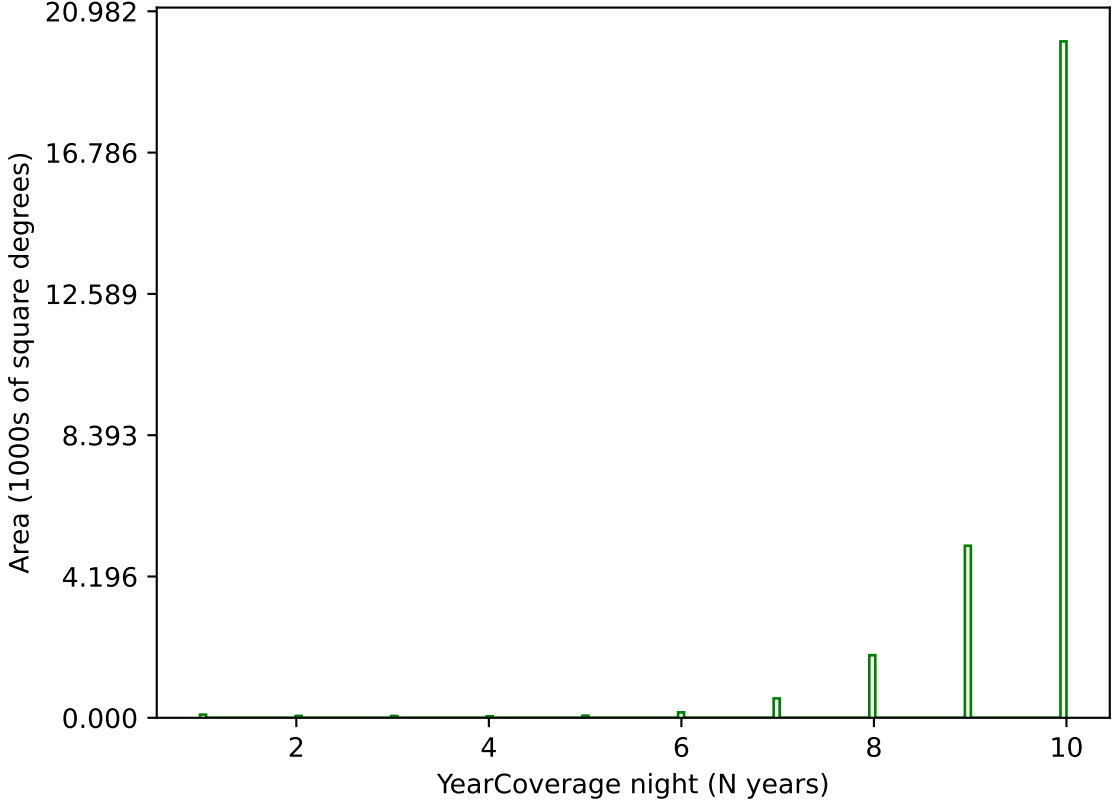
weather_cloudso31v3.4_10yrs g band: YearCoverage night
