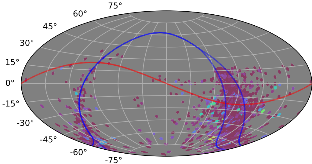
weather_cloudso31v3.4_10yrs : XRBPpopMetric_number_of_detections
