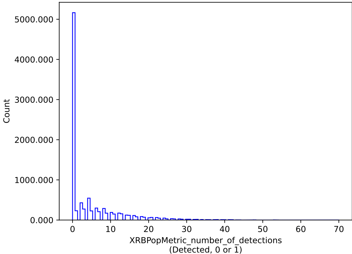
weather_cloudso31v3.4_10yrs : XRBPoMetric_number_of_detections
