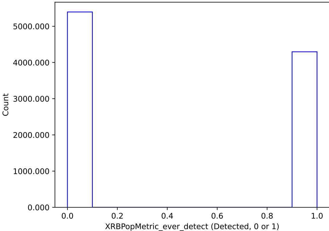
weather_cloudso31v3.4_10yrs : XRBPoMetric_ever_detect
