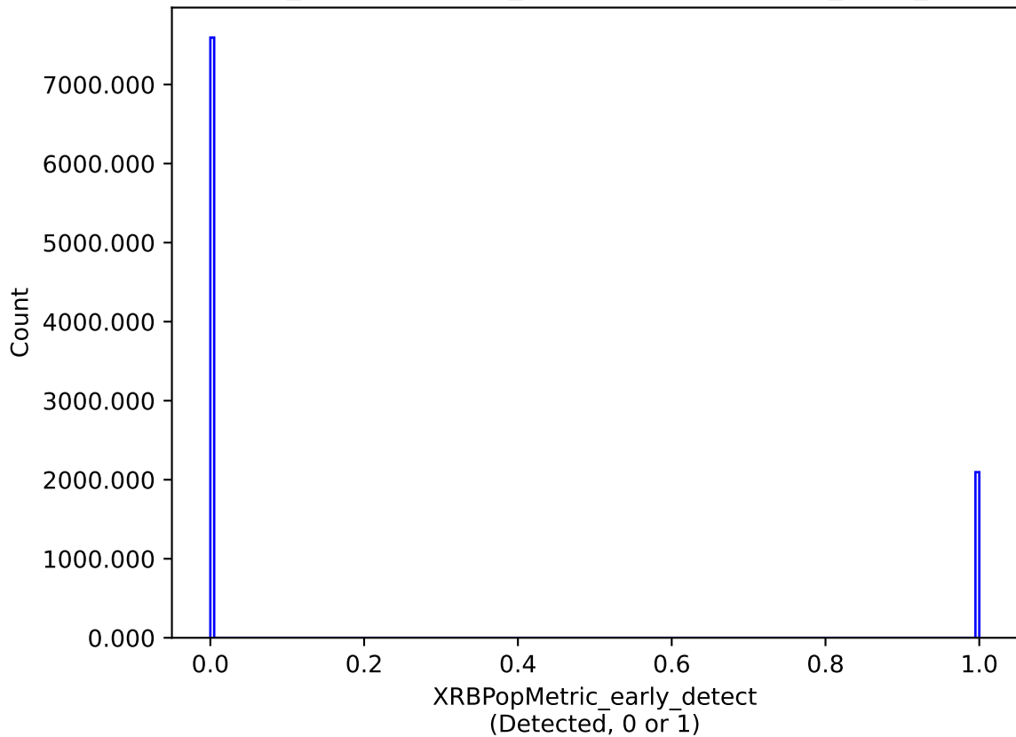
weather_cloudso31v3.4_10yrs : XRBPoMetric_early_detect
