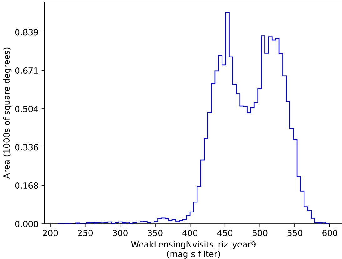
weather_cloudso31v3.4_10yrs gri band non-DD: WeakLensingNvisits_riz_year9
