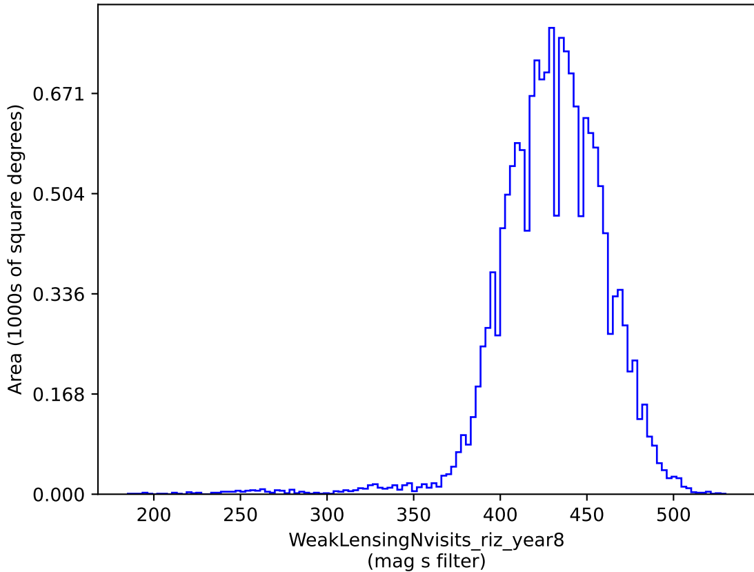
weather_cloudso31v3.4_10yrs gri band non-DD: WeakLensingNvisits_riz_year8
