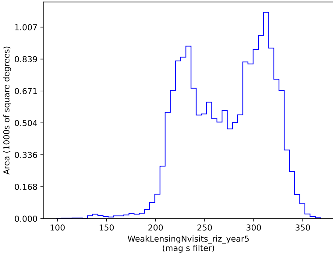
weather_cloudso31v3.4_10yrs gri band non-DD: WeakLensingNvisits_riz_year5
