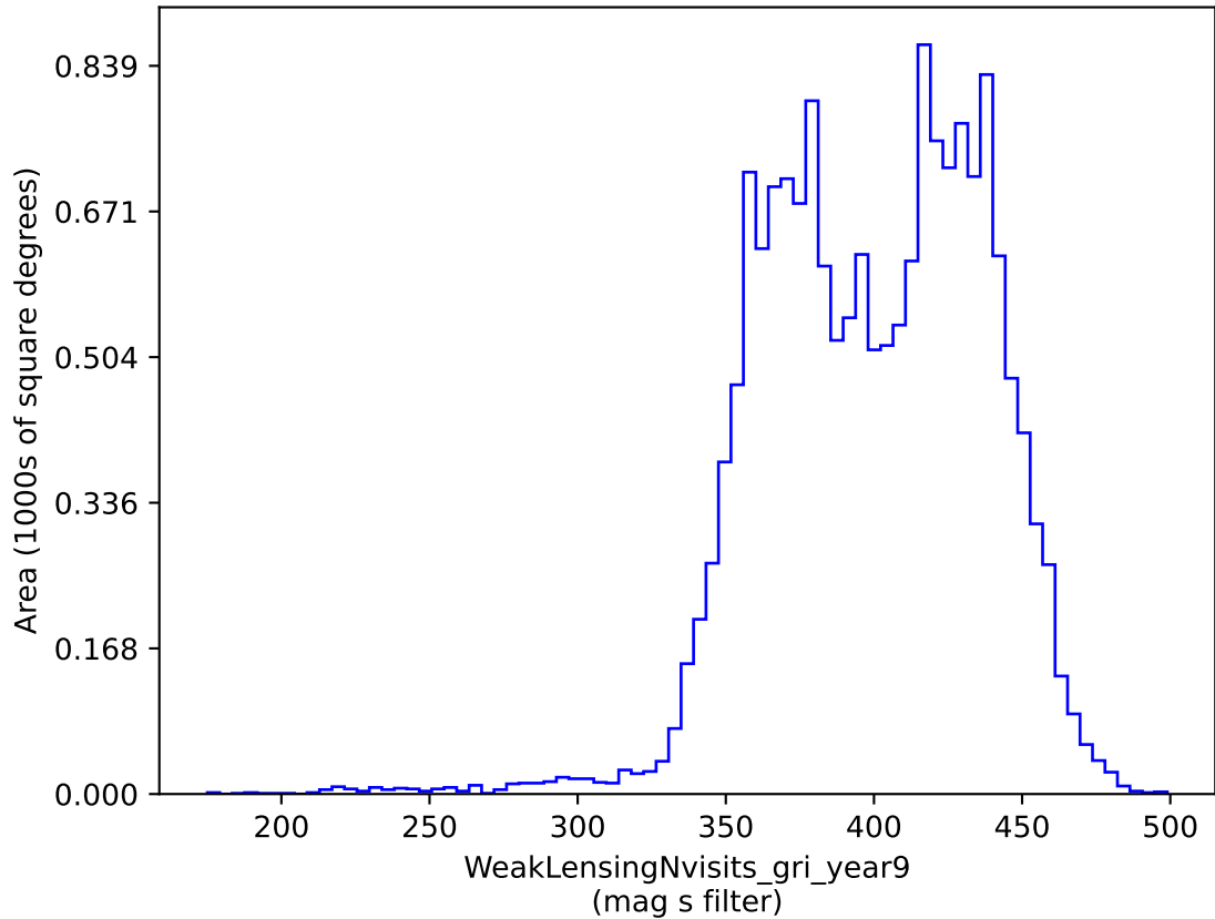
weather_cloudso31v3.4_10yrs gri band non-DD: WeakLensingNvisits_gri_year9
