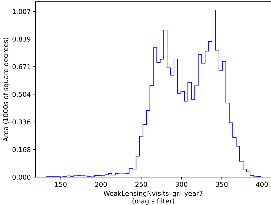
weather_cloudso31v3.4_10yrs gri band non-DD: WeakLensingNvisits_gri_year7
