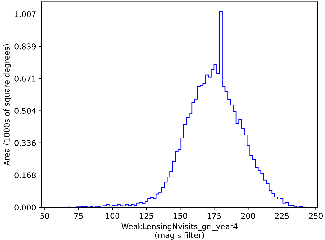
weather_cloudso31v3.4_10yrs gri band non-DD: WeakLensingNvisits_gri_year4
