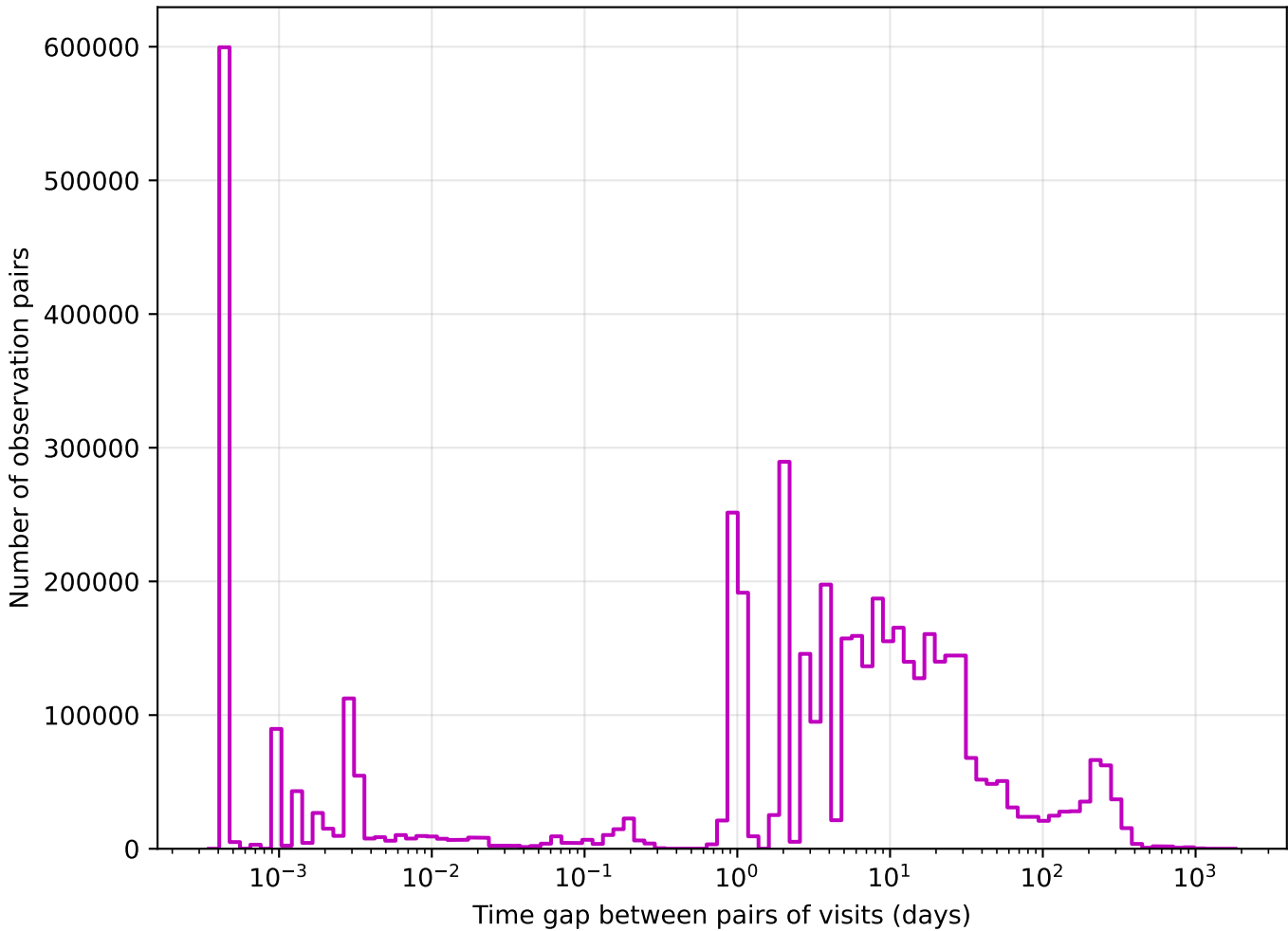
weather_cloudso31v3.4_10yrs z band: Tgaps observationStartMJD
