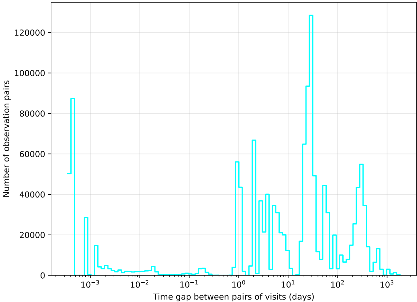
weather_cloudso31v3.4_10yrs u band: Tgaps observationStartMJD
