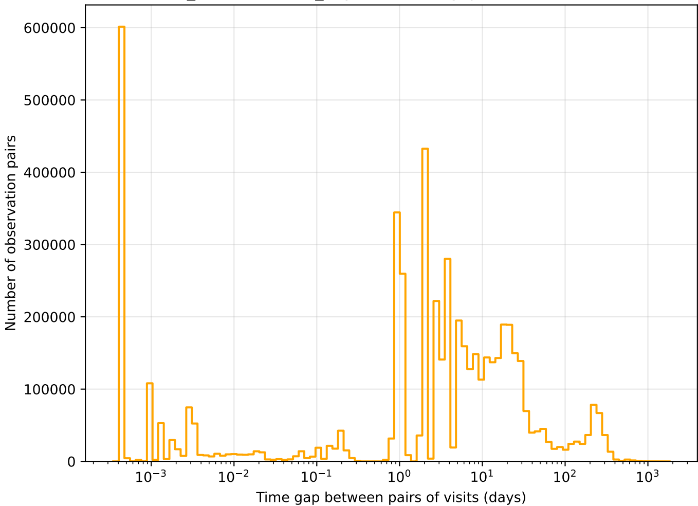
weather_cloudso31v3.4_10yrs r band: Tgaps observationStartMJD
