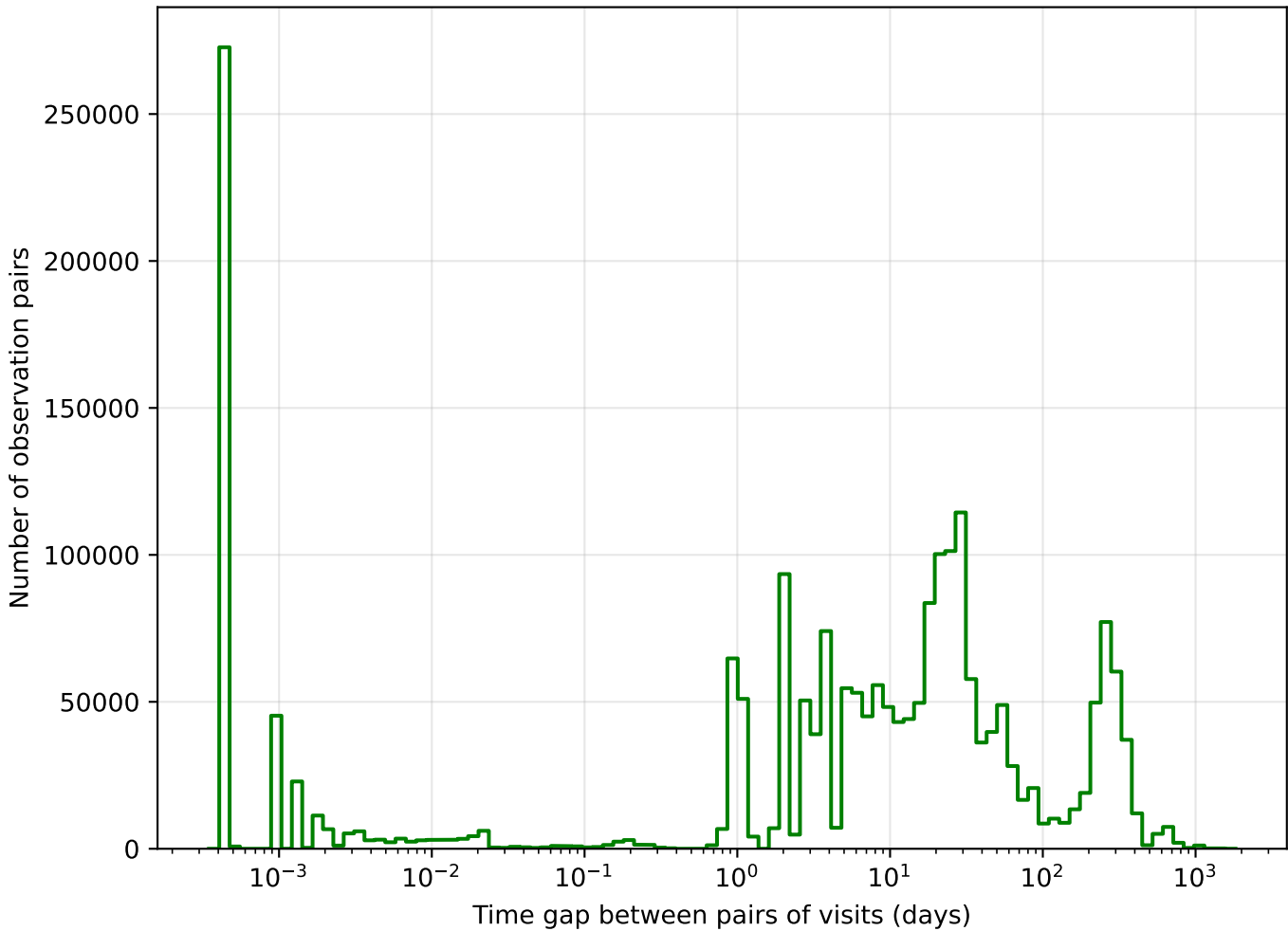
weather_cloudso31v3.4_10yrs g band: Tgaps observationStartMJD
