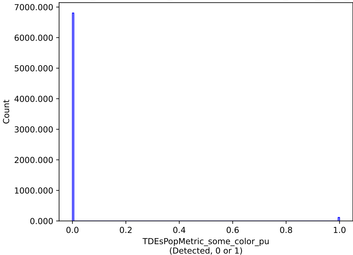
weather_cloudso31v3.4_10yrs : TDEsPopMetric_some_color_pu
