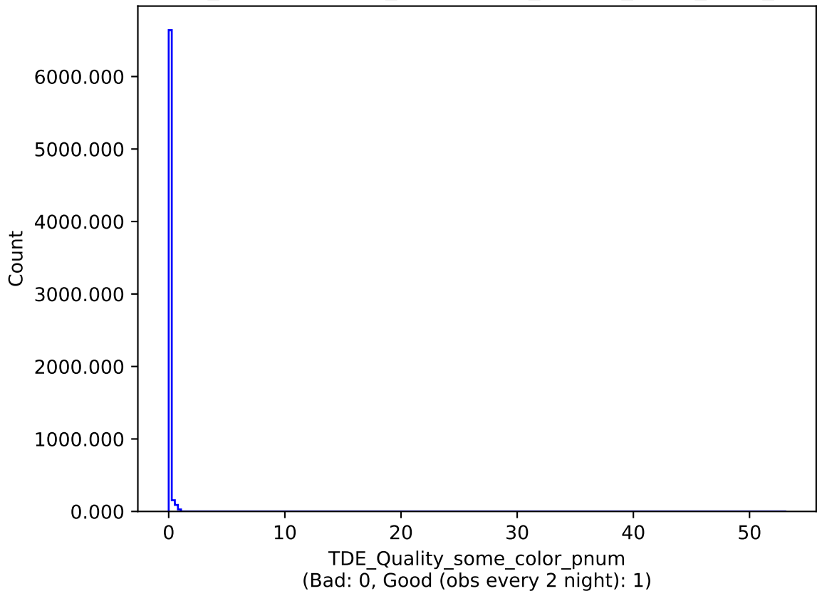
weather_cloudso31v3.4_10yrs : TDE_Quality_some_color_pnum
