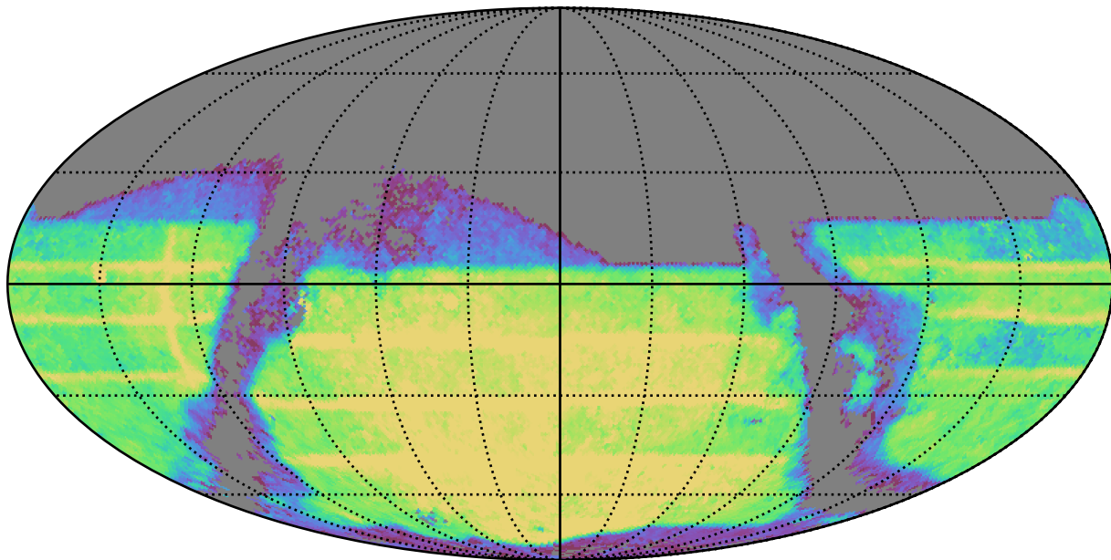
weather_cloudso31v3.4_10yrs : TDC_rate
