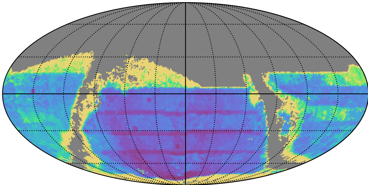
weather_cloudso31v3.4_10yrs : TDC_accuracy
