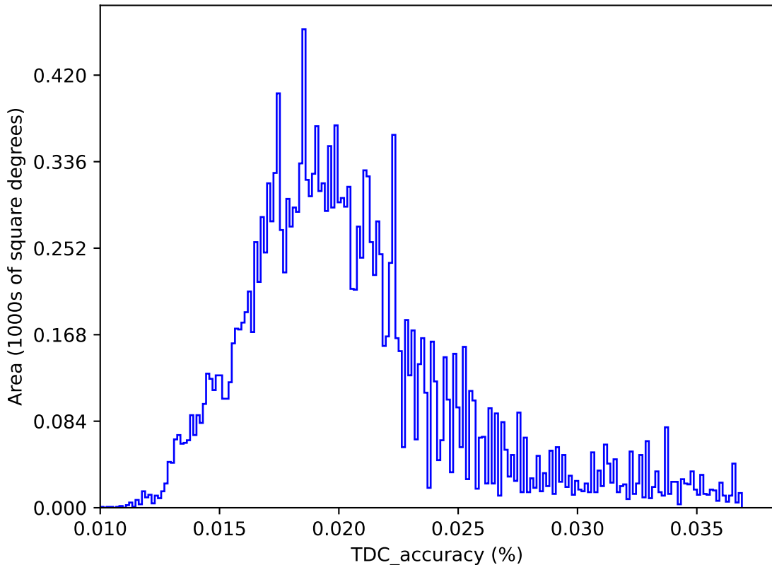
weather_cloudso31v3.4_10yrs : TDC_accuracy
