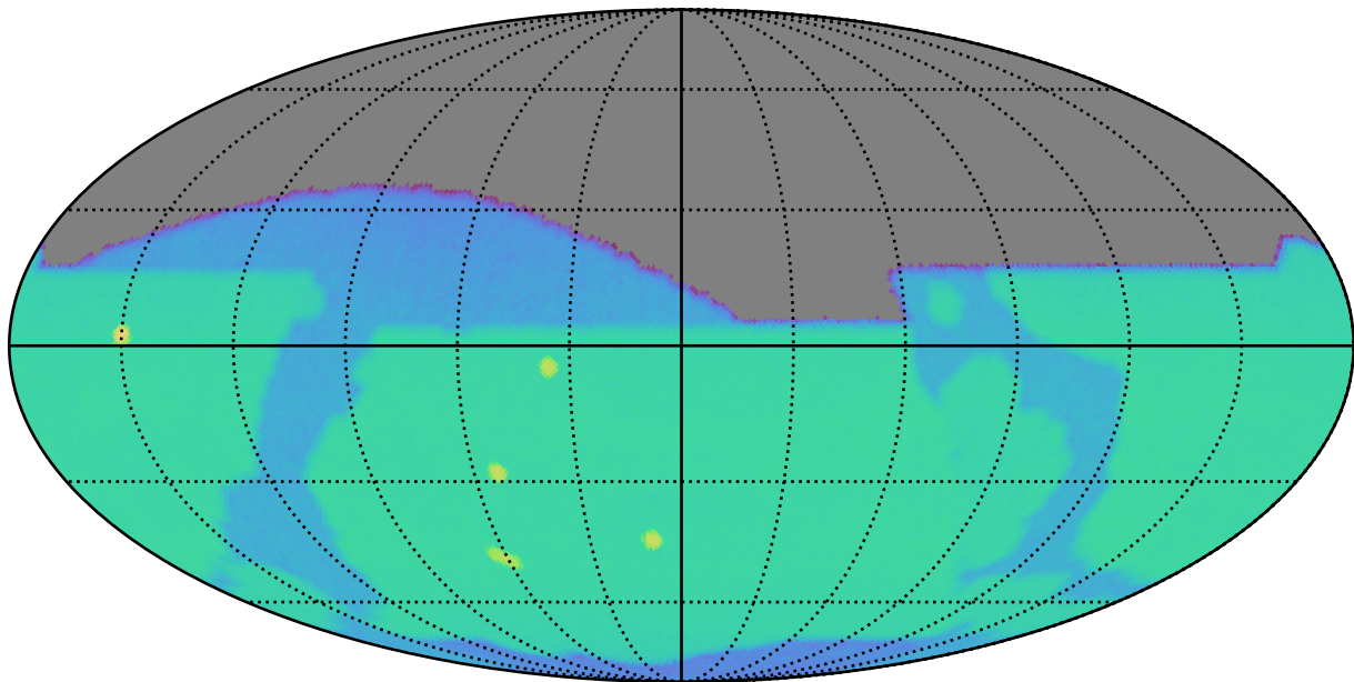
weather_cloudso31v3.4_10yrs z: SurfaceBrightLimit
