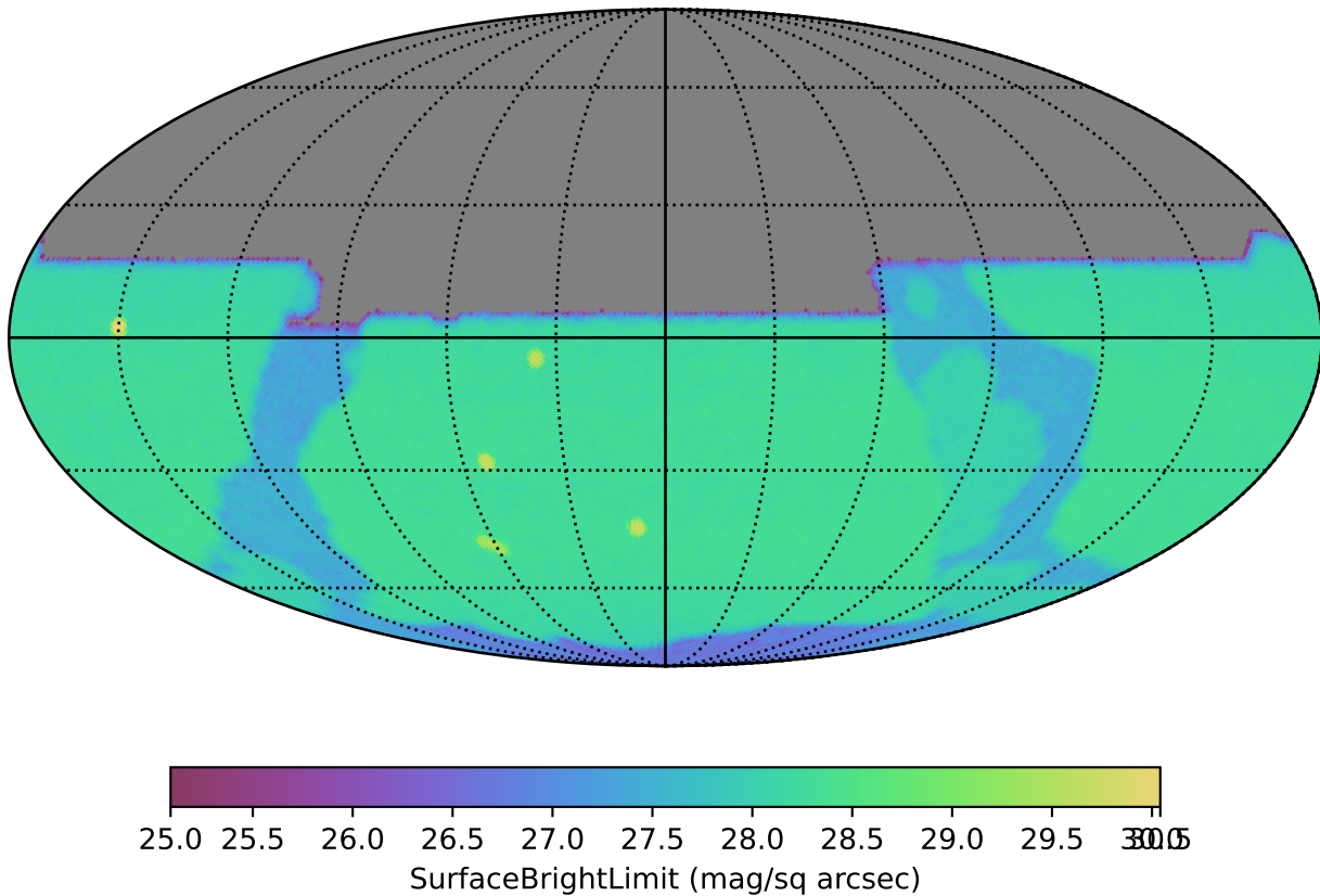
weather_cloudso31v3.4_10yrs y: SurfaceBrightLimit
