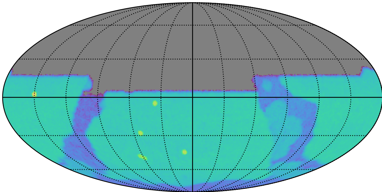
weather_cloudso31v3.4_10yrs u: SurfaceBrightLimit
