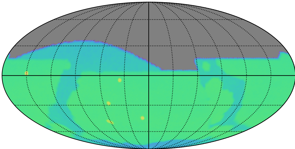
weather_cloudso31v3.4_10yrs r: SurfaceBrightLimit
