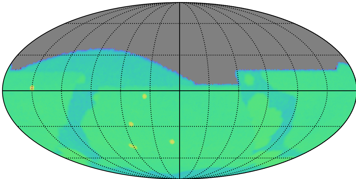
weather_cloudso31v3.4_10yrs g: SurfaceBrightLimit
