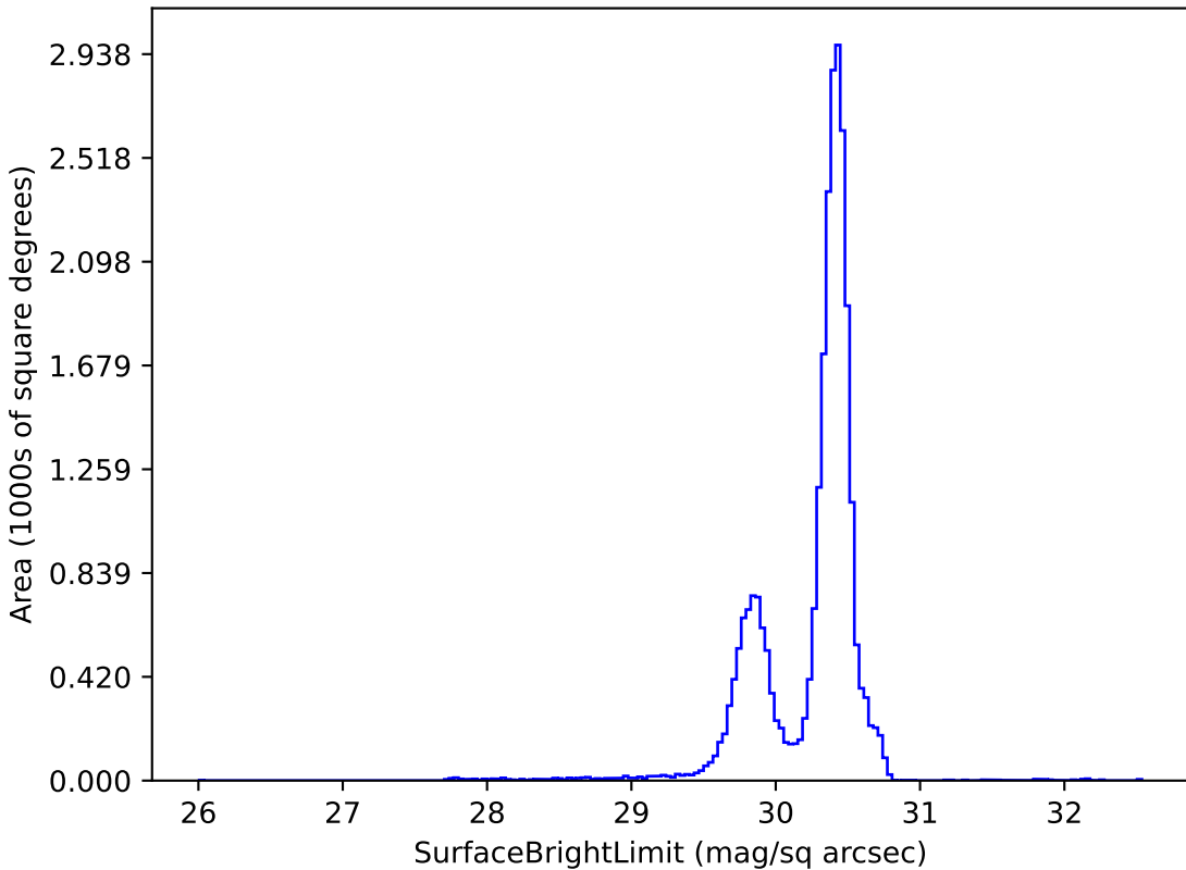
weather_cloudso31v3.4_10yrs g: SurfaceBrightLimit
