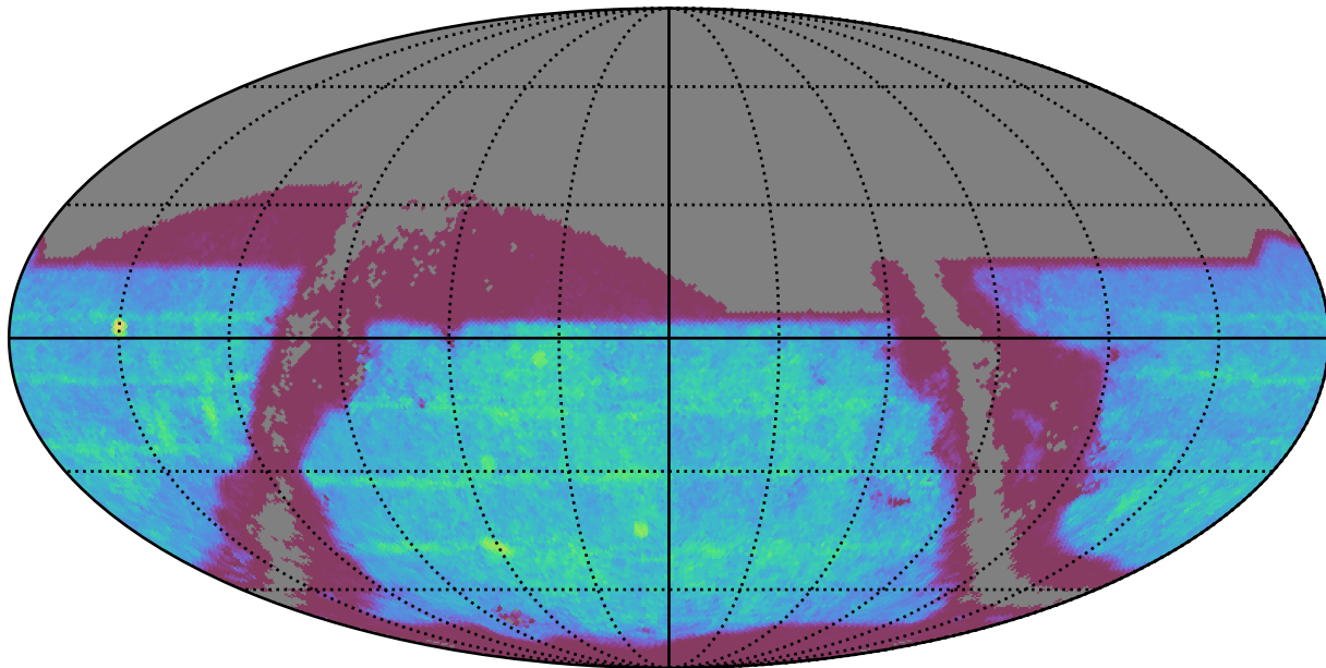
weather_cloudso31v3.4_10yrs : SNSLMetric
