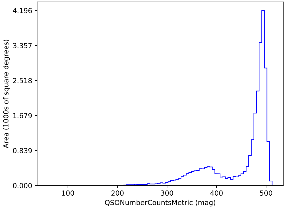
weather_cloudso31v3.4_10yrs z band and non-DD: QSONumberCountsMetric
