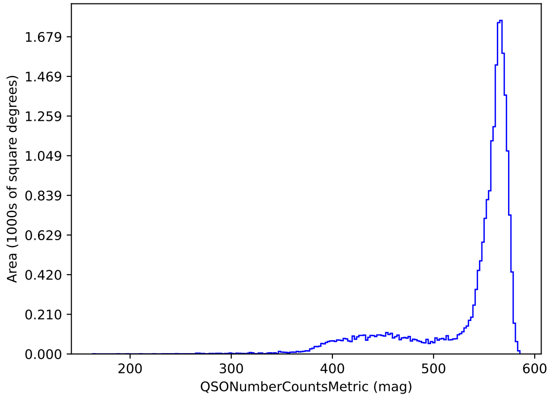
weather_cloudso31v3.4_10yrs y band and non-DD: QSONumberCountsMetric
