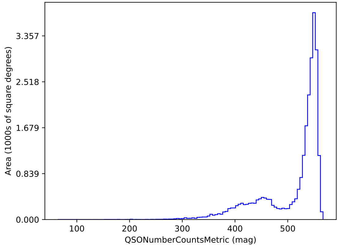
weather_cloudso31v3.4_10yrs i band and non-DD: QSONumberCountsMetric
