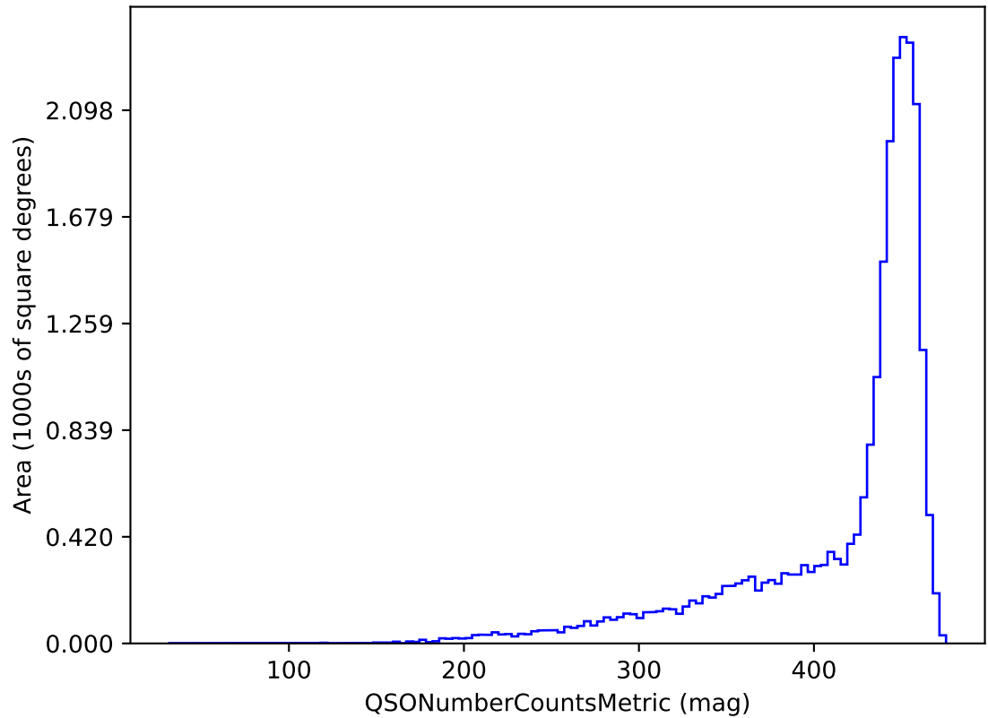
weather_cloudso31v3.4_10yrs g band and non-DD: QSONumberCountsMetric
