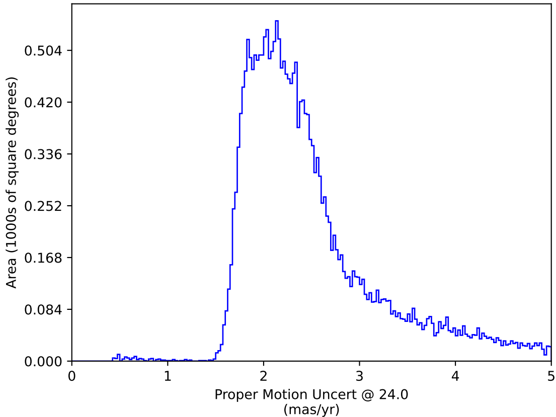
weather_cloudso31v3.4_10yrs : Proper Motion Uncert @ 24.0
