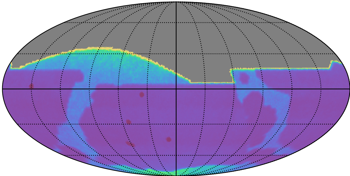
weather_cloudso31v3.4_10yrs : Proper Motion Uncert @ 20.5
