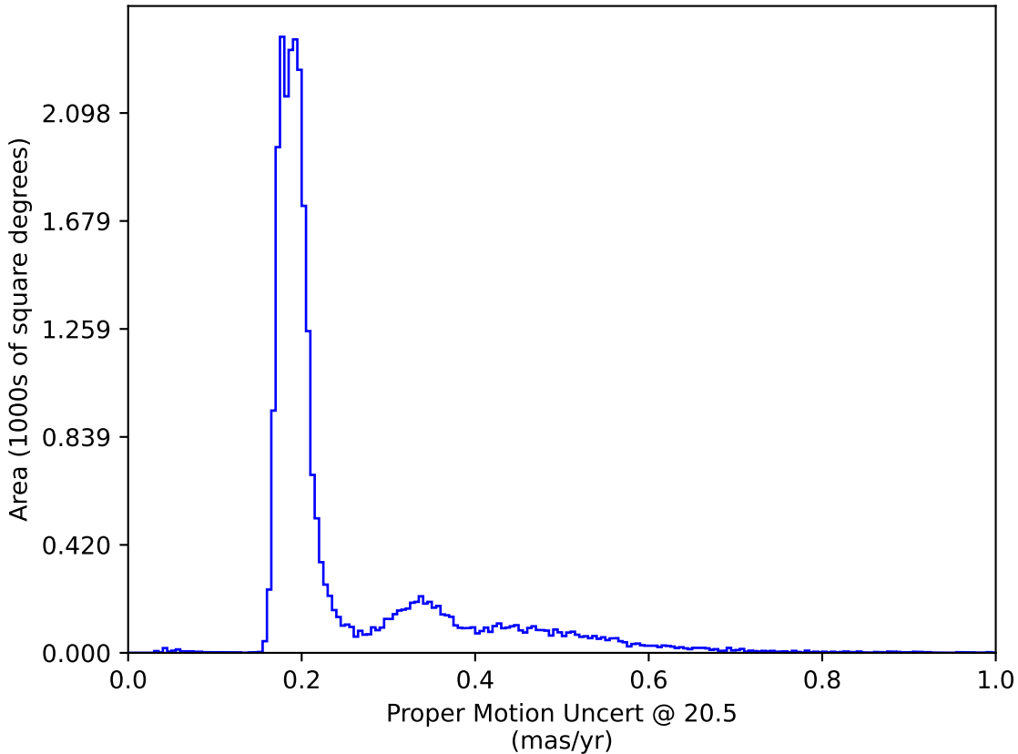
weather_cloudso31v3.4_10yrs : Proper Motion Uncert @ 20.5
