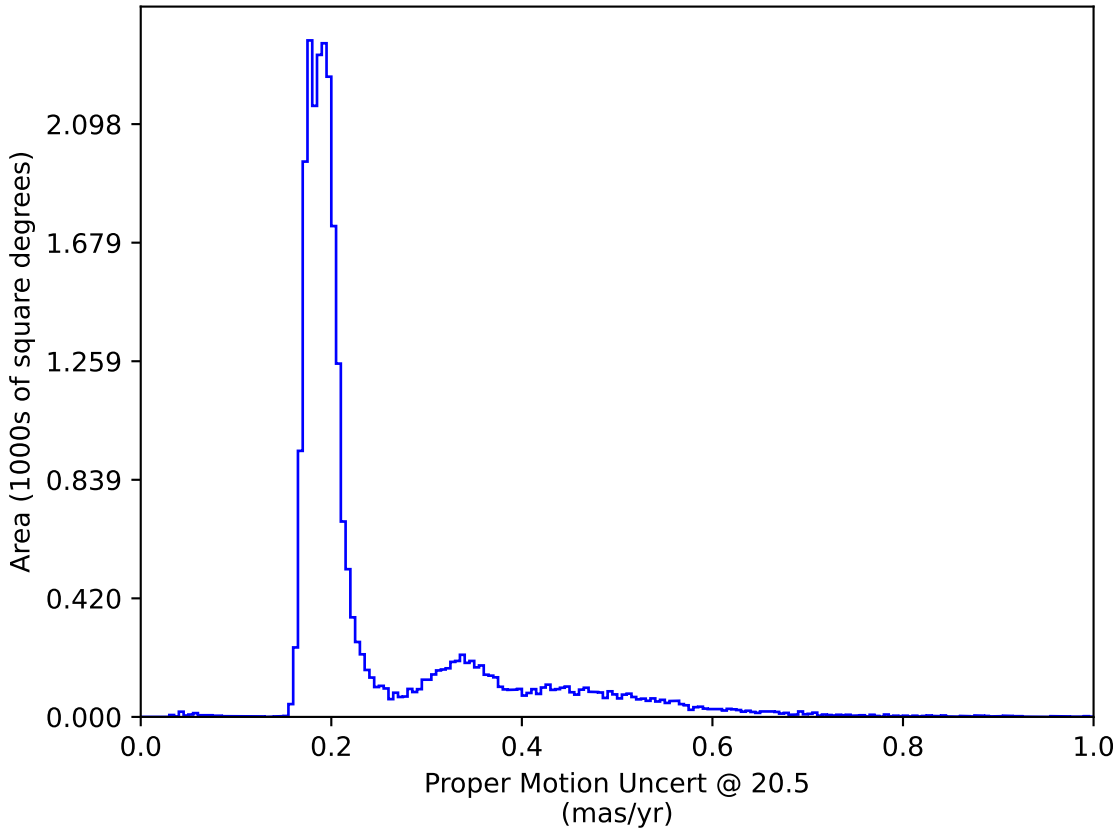
weather_cloudso31v3.4_10yrs : Proper Motion Uncert @ 20.5
