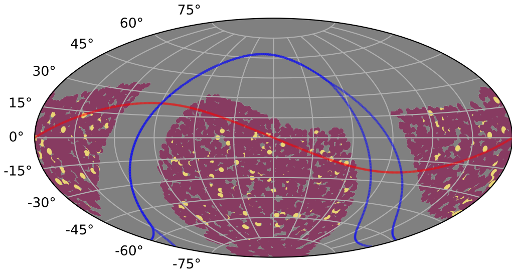
weather_cloudso31v3.4_10yrs : PrestoKNe_score_s
