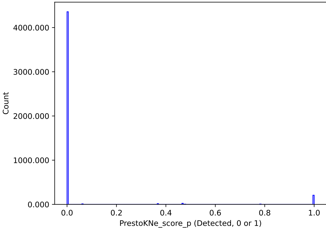
weather_cloudso31v3.4_10yrs : PrestoKNe_score_p
