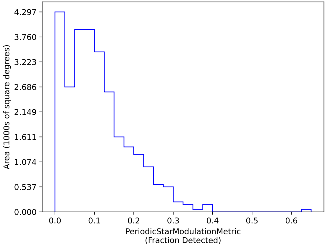
weather_cloudso31v3.4_10yrs dm 19 interval 15 RRC Year 1-2: PeriodicStarModulationMetric
